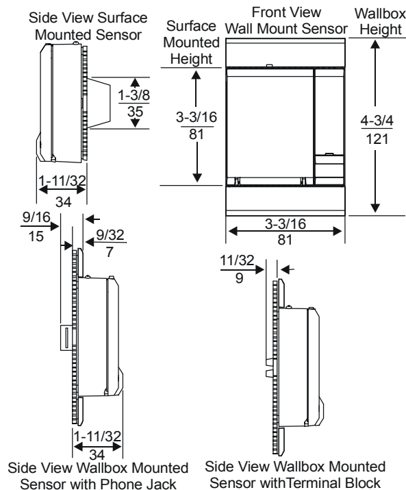
Figure 2: TE-6700 Dimensions, in. (mm)
