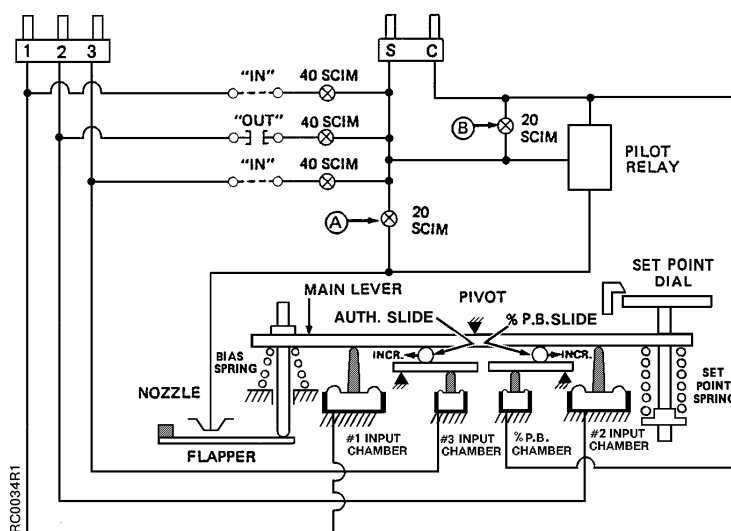
Figure 1. Multiple Input Receiver-Controller Schematic.
