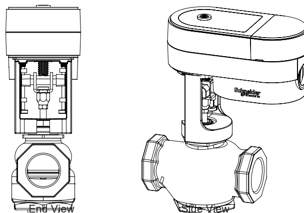
MG350V Installed on a VB-7000 Globe Valve
