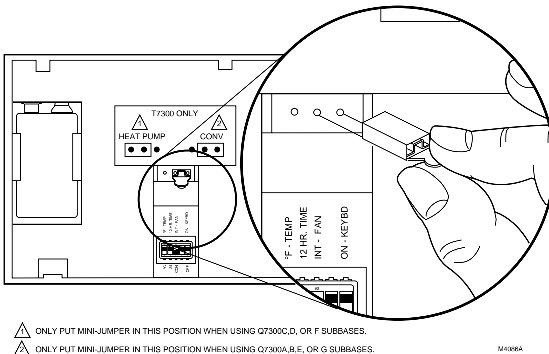
Fig. 14—Setting thermostat mini-jumper for conventional or heat pump system.
