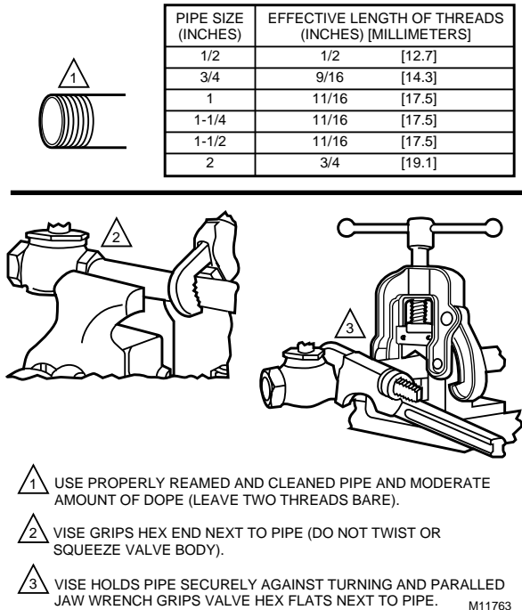
Fig. 8. Installing valves with threaded connections.
