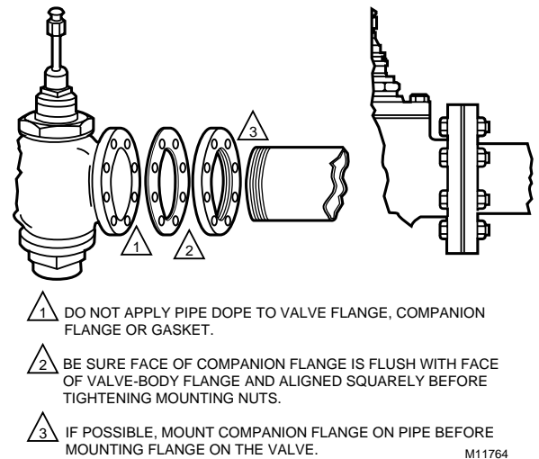
Fig. 9. Proper flange mounting.
