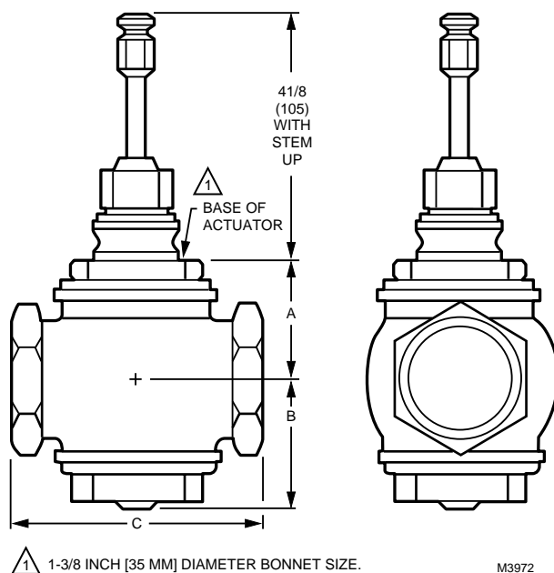
Fig. 7. V5011H,J threaded, reverse acting body dimensions. See Table 2.
